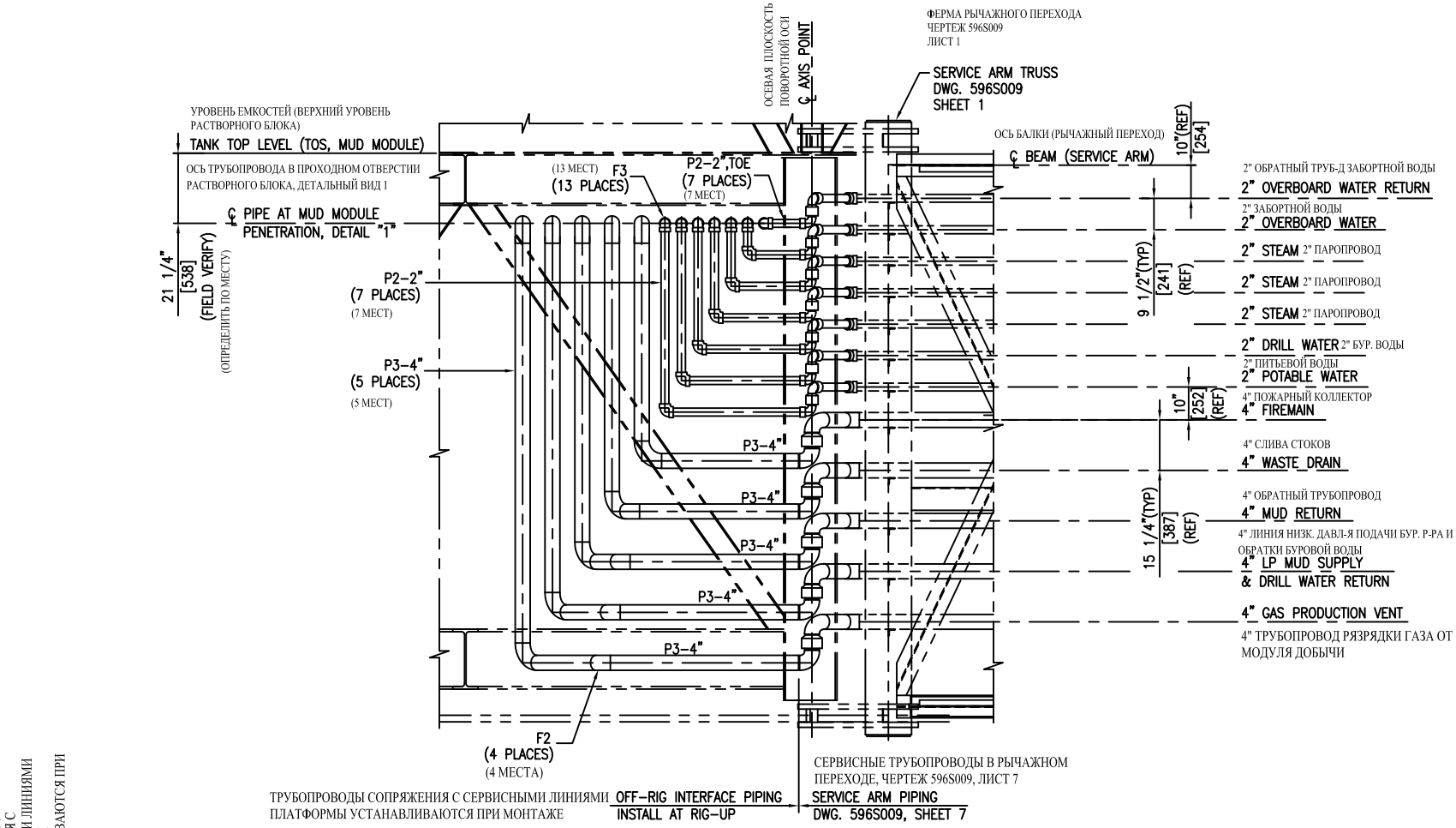
SECTION "1-1" OFF-RIG UTILITY PIPING СЕЧЕНИЕ 1-1
