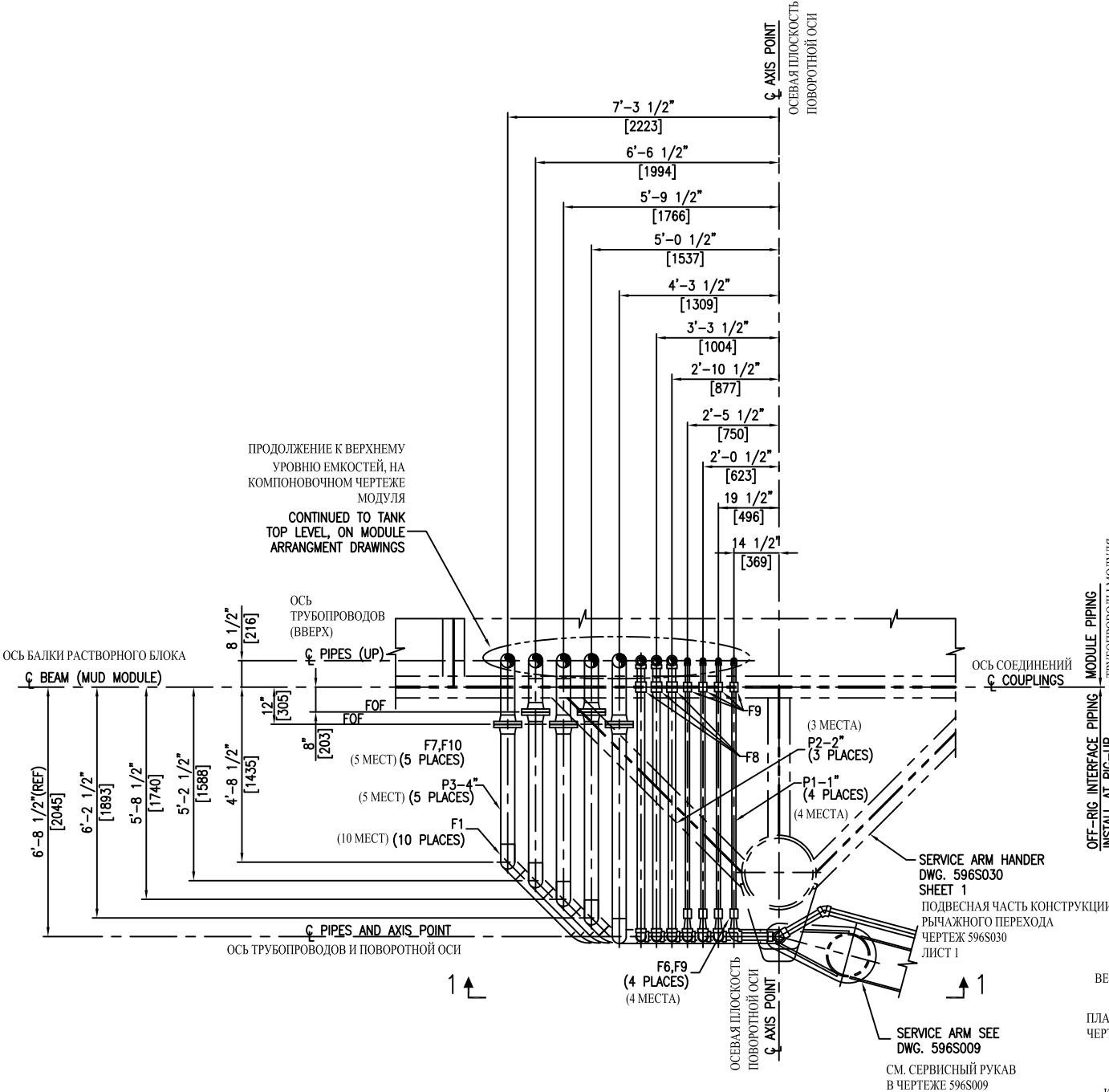
PLAN VIEW—PUMP LEVEL OFF-RIG UTILITY PIPING
